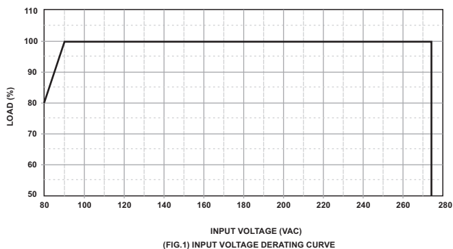
(FIG.1) INPUT VOLTAGE DERATING CURVE
