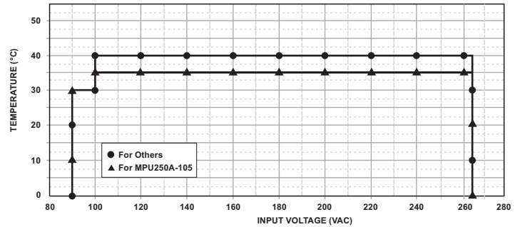
(FIG.2) TEMPERATURE DERATING CURVE
