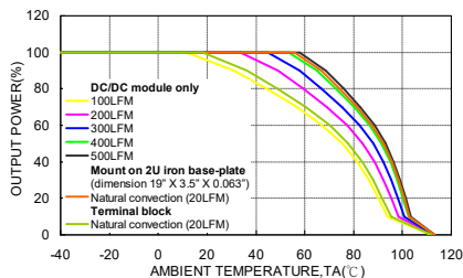
HAE200-48S05 Derating Curve (See Thermal Considerations)
