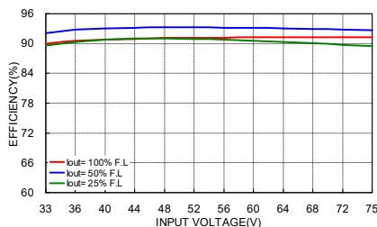
HAE200-48S05 Efficiency vs. Input Voltage
