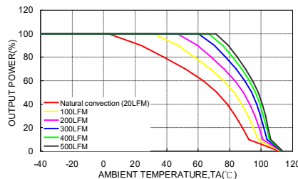
HAE200-48S05 Derating Curve With 0.24" Height Heat-sink (See Thermal Considerations)
