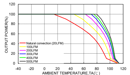
HAE200-48S05 Derating Curve With 0.45" Height Heat-sink (See Thermal Considerations)
