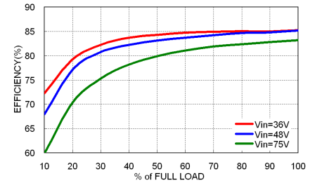
MOP06-48S05WA Efficiency vs. Output Load
