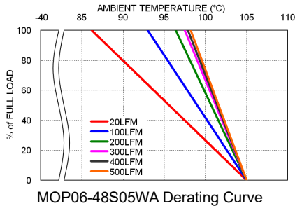
MOP06-48S05WA Derating Curve
