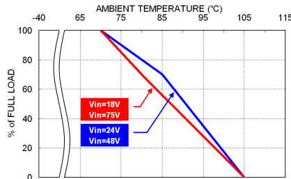
RCD15-48□□□W Derating Curve
