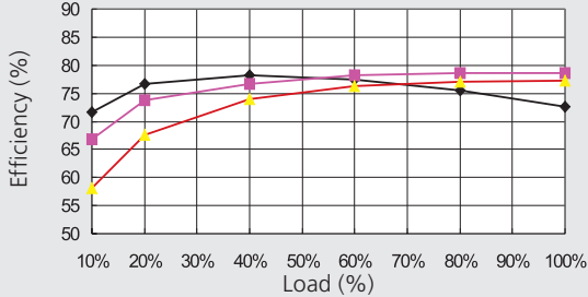
RRD-4805S06AXW Efficiency vs Output Current
