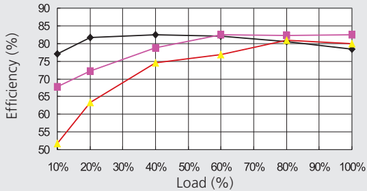
RRD-4805S06AXW Efficiency vs Output Current
