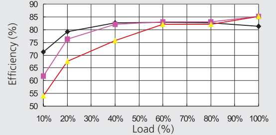
RRD-4824D06AXW Efficiency vs Output Current
