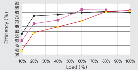
RRD-4824D06AXW Efficiency vs Output Current
