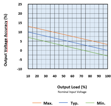
12V & 24V input with 12V & 15V output
