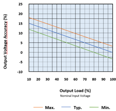
12V & 24V input with 3.3V & 5V output
