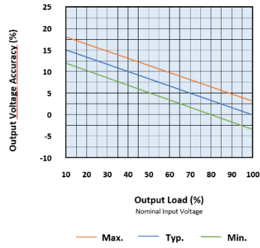
5V input with 12V & 15V output
