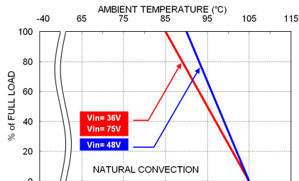
MPS(H)02-48□□□ Derating Curve
