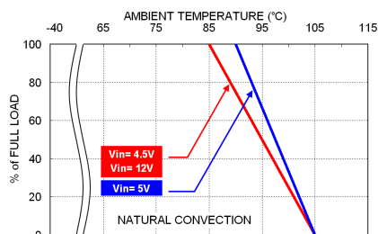
MPS(H)02-05□□□ Derating Curve
