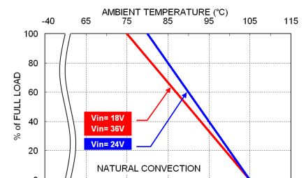
MPS(H)04-24□□□ Derating Curve
