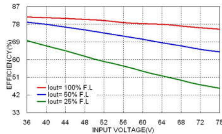
SDS(H)02-48S05 Efficiency vs. Input Voltage
